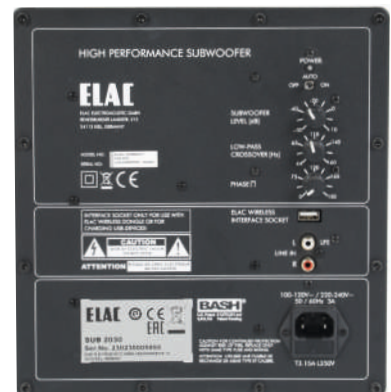
Rearview SUB 2030
